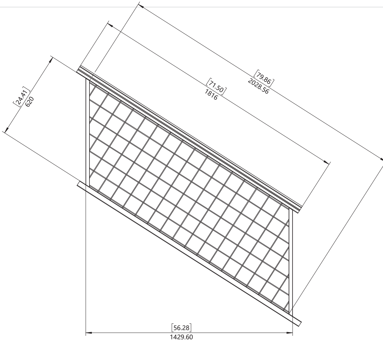
36" x 72" Mesh Stair Railing
